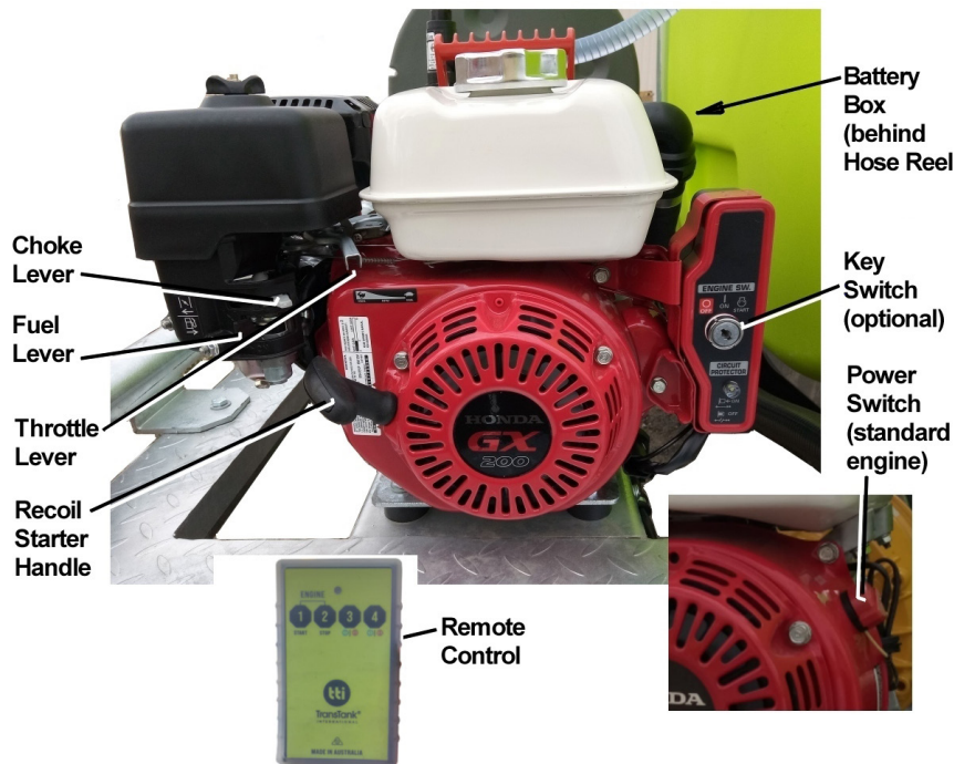
Figure 3 – Engine Start-up (Petrol Engine shown)
