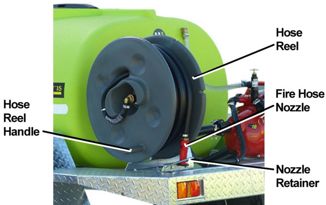
Figure 6 – Fire Hose Reel
