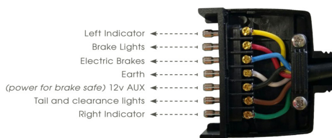
7-Pin Plug Wiring Requirements
