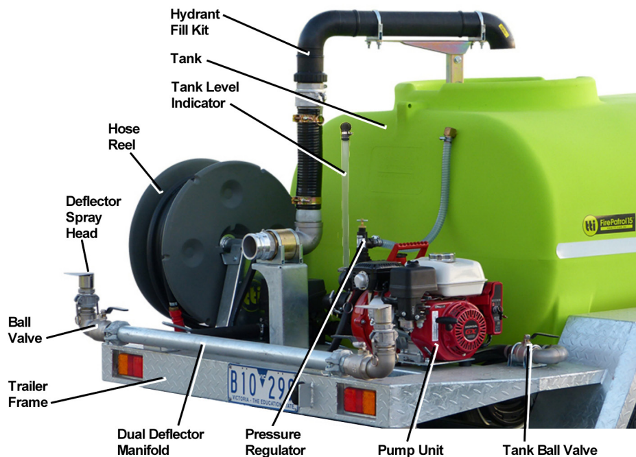
Figure 1 – Component Identification
