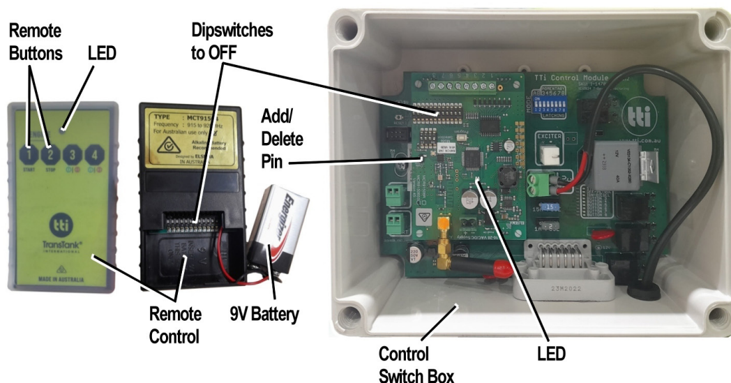
Figure 9 – Control Switch and Remote Control
