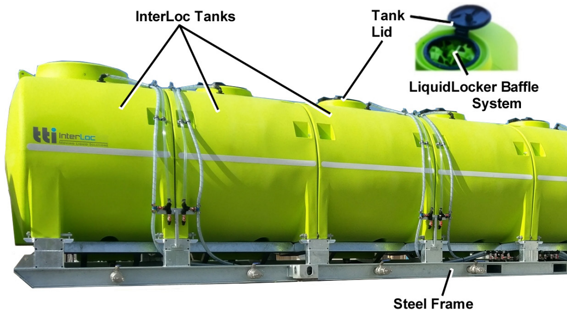
Figure 2 – InterLoc Component Identification
