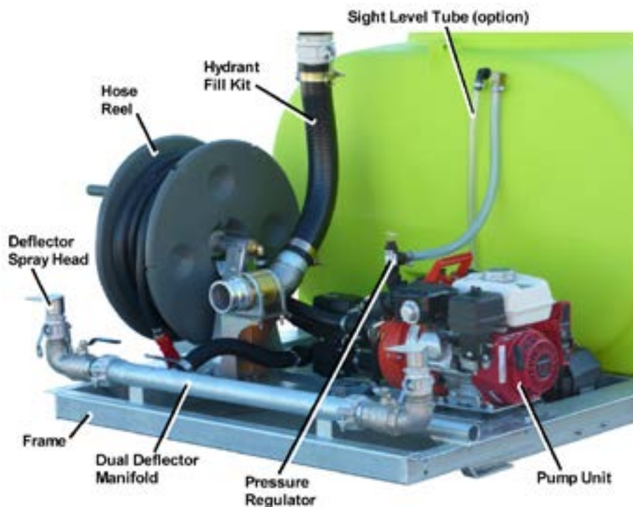
Figure 2 – Component Identification
