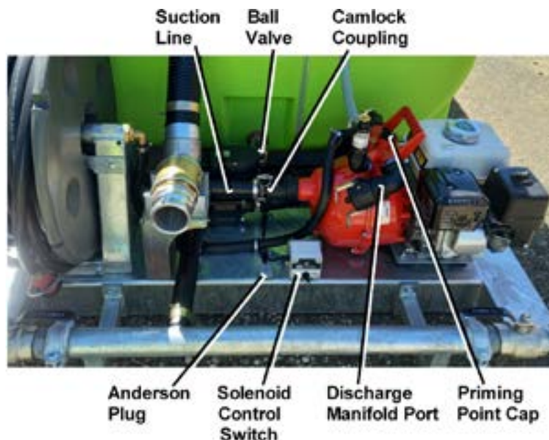
Figure 5 – Tank Filling Operation
