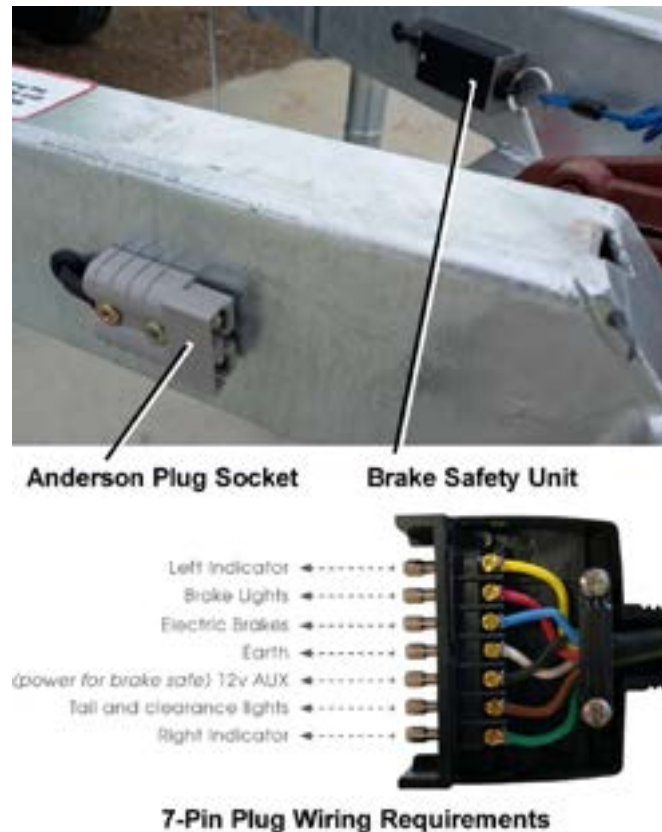
Figure 3 – Coupling Brake Unit – xTreme variant
