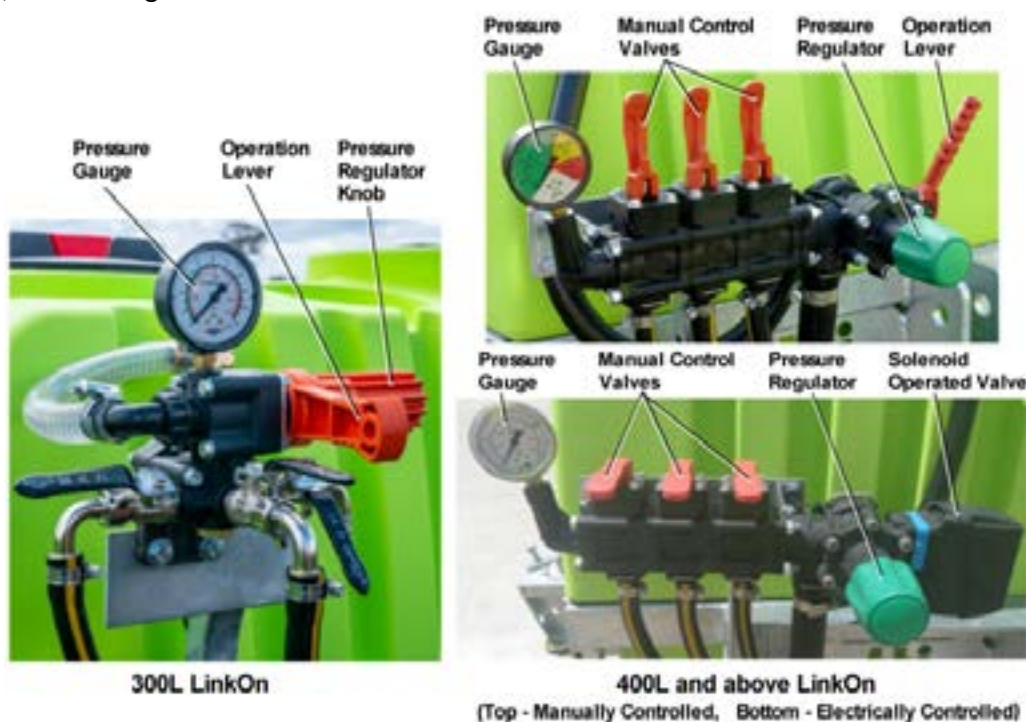
Figure 5 – Pressure Regulator
