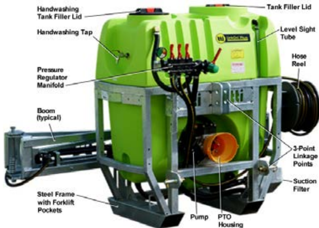
Figure 1 – Component Identification – LinkOn with hose reel option
