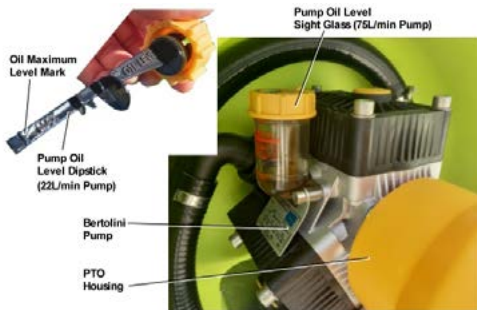
Figure 10 – Bertolini Pump
